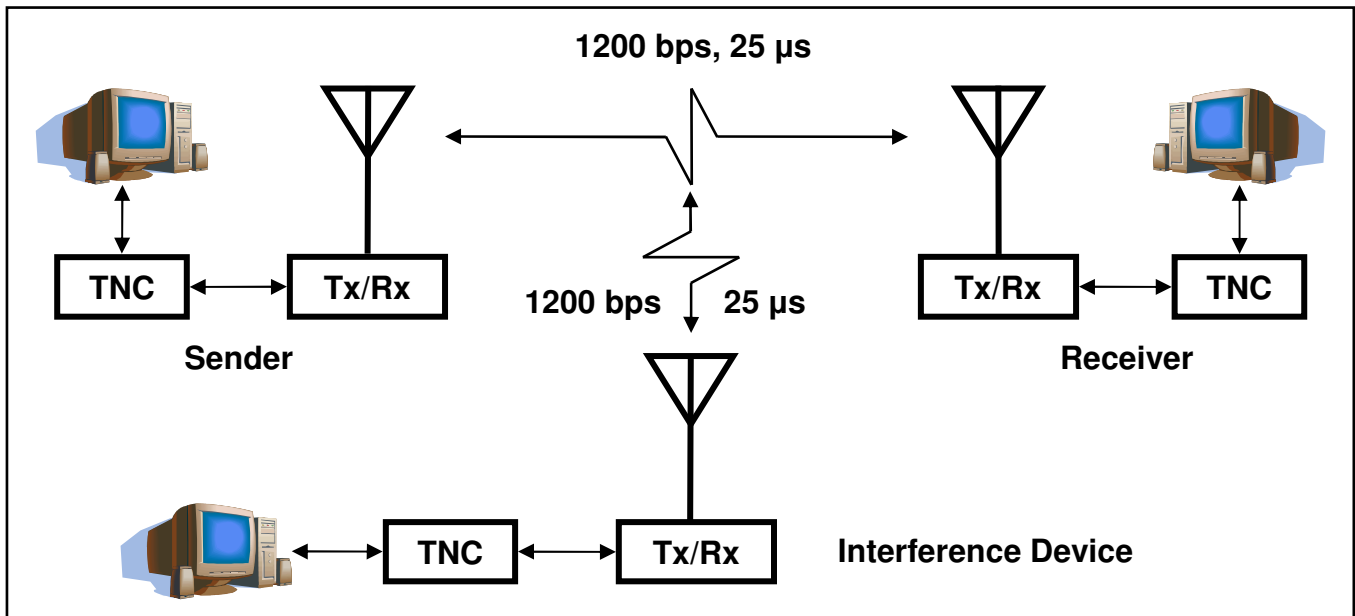
Figure 2: An Example 3 Node, 1 Link Packet Radio Network.
